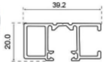
AP Self-supporting slide
