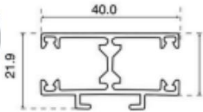
DPF Double face-mounted slide
