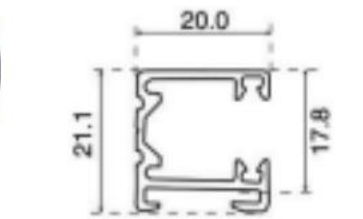
SFP Single slide, face-mounted and table-mounted
